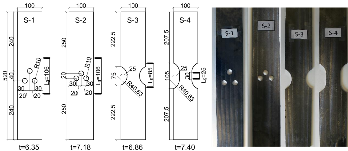
Figure 3.10. Configuration of the pull-plate test specimens tested and simulated by calibrated numerical models.
