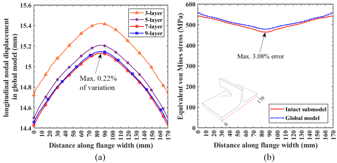
Fig. 10. Mesh sensitivity analysis result at the boundary of submodel region: a) Longitudinal nodal displacement of global model converged by using seven layers of elements through the thickness of the plates, b) Comparison between stress values obtained from the global model and submodel.
