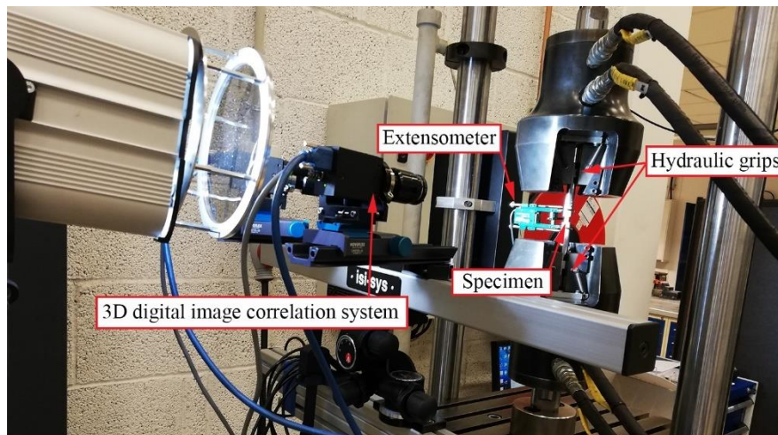
Figure 3.6. Test setup configuration for round bar specimens.
